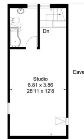
Garage - First Floor
